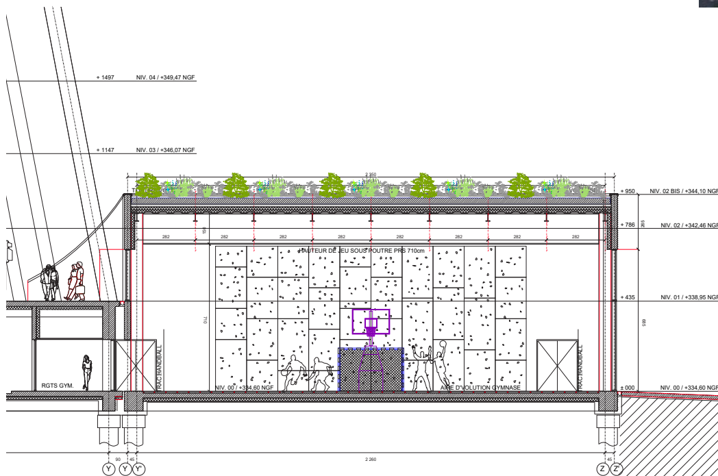
COUPE TRANSVERSALE AA - PHASE 1 - CH. 1/100°
